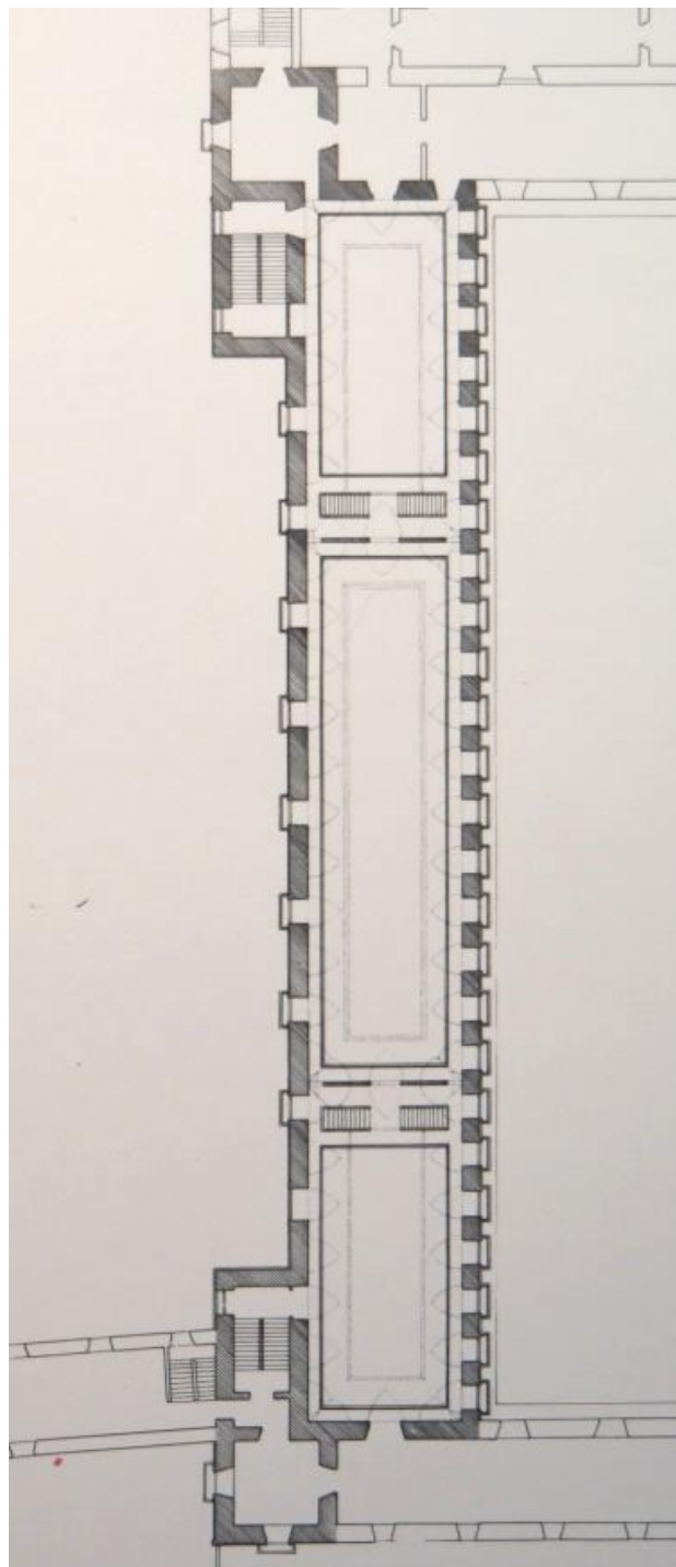
Floor plan of Hall of Realms (left) and plan of perimetric gallery. 1640. (Research of Carmen Blasco).
